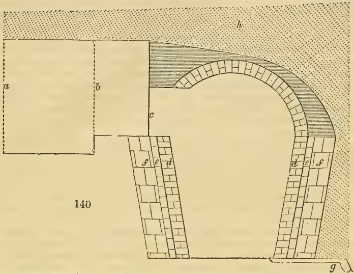
a, Front oak door. b, Second door. c, Sliders, coming out one board at a time. d, 9-inch brick wall. e, 4½-inch cavity. f, 14-inch stone wall. g, 3-inch drains. h, Soil on top
